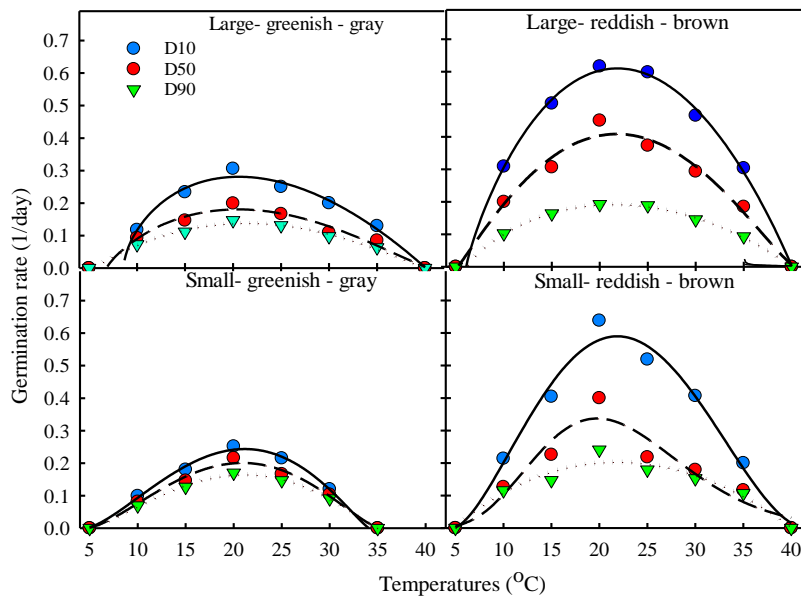
Figure 2. Predicted (lines) vs. observed (symbols) germination rate of Ricinus communis seeds at different constant temperatures using non-linear models.
