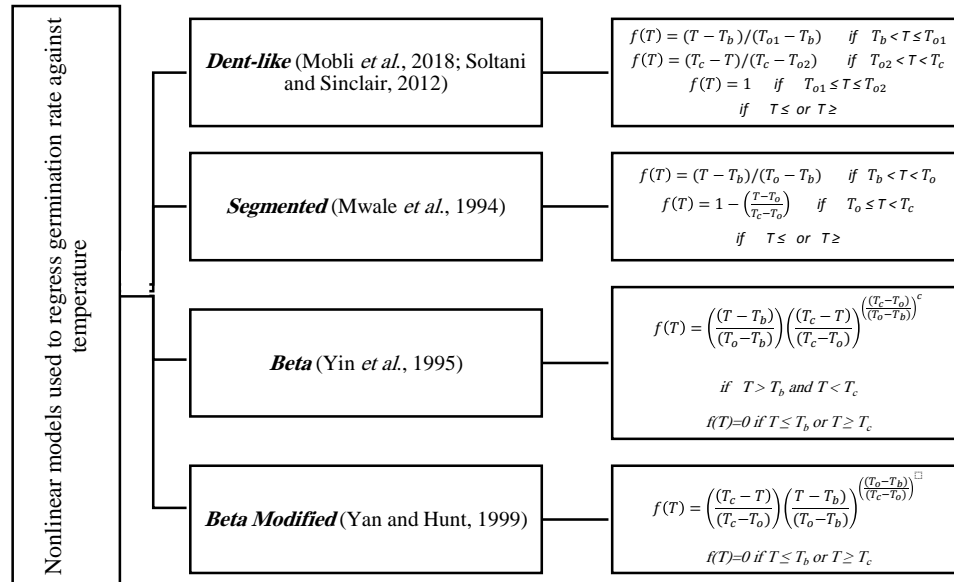
Figure 1. Nonlinear models used to regress germination rate against temperature.
