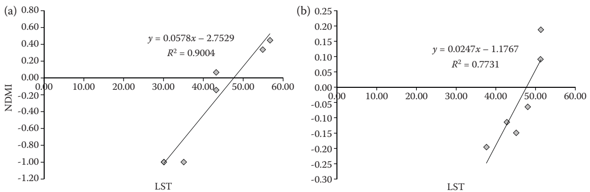
Fig. 5. Regression between normalized difference moisture index (NDMI) and land surface temperature (LST) using Landsat 8 (a), Moderate Resolution Imaging Spectroradiometer – MODIS (b)
